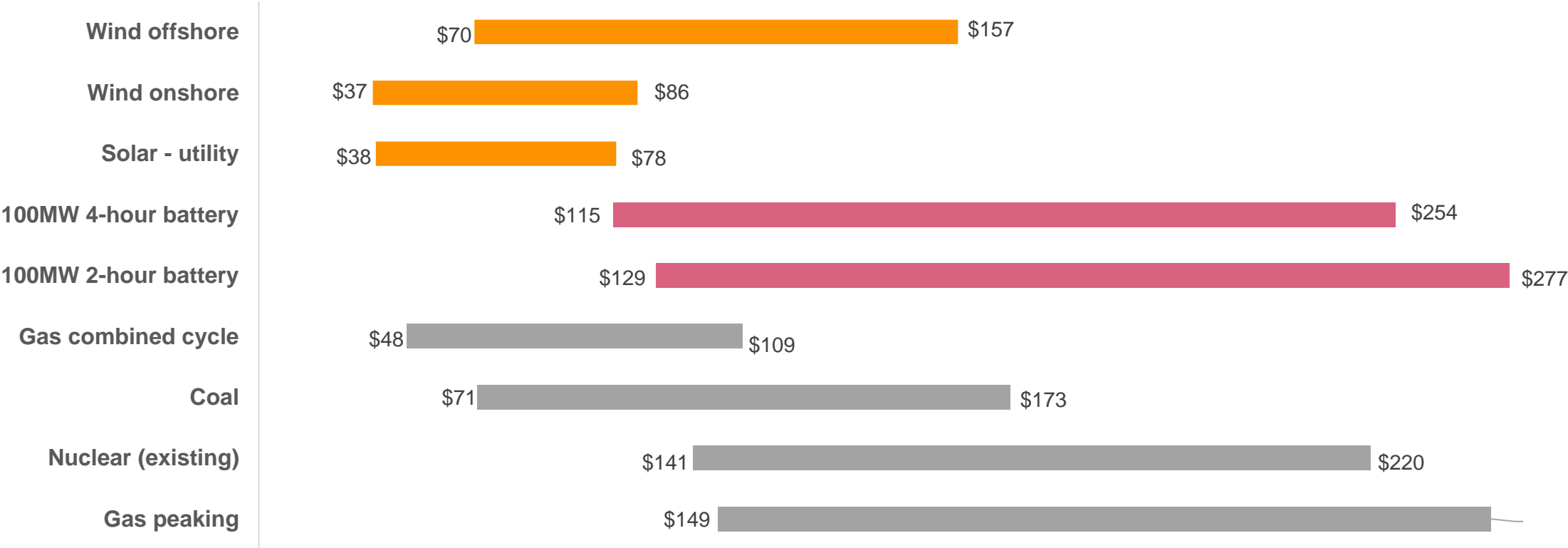
Levelised cost of United States energy/storage (US$/MWh)
