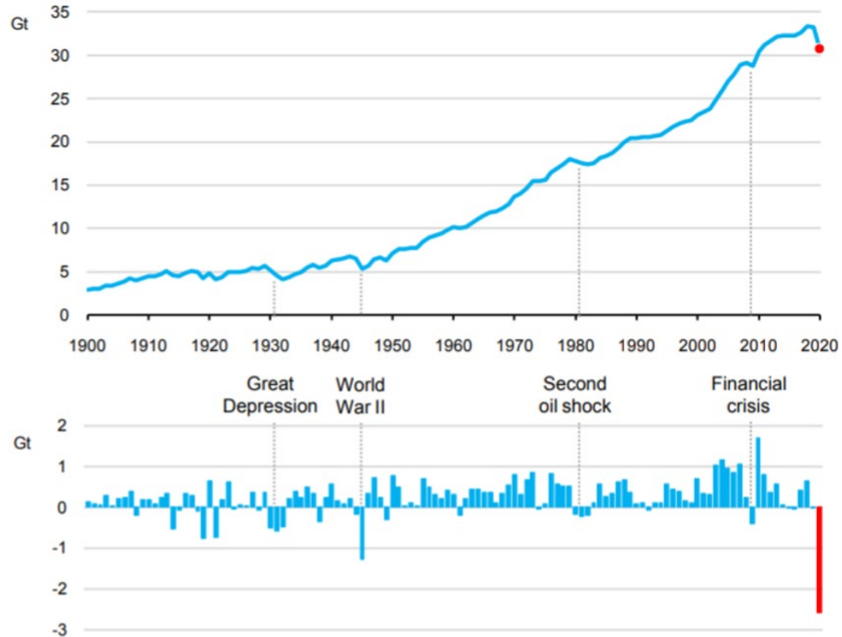
Global Energy Related CO2 Emissions & Annual Change
